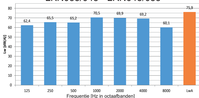
LKN035/045 - LRN045/055
